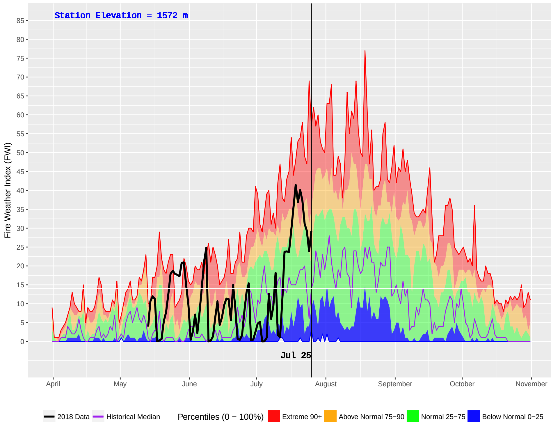
NEGRO CREEK (789) : Historical (2001–2016) and Current (2018) Noon Fire Weather Index (FWI)
