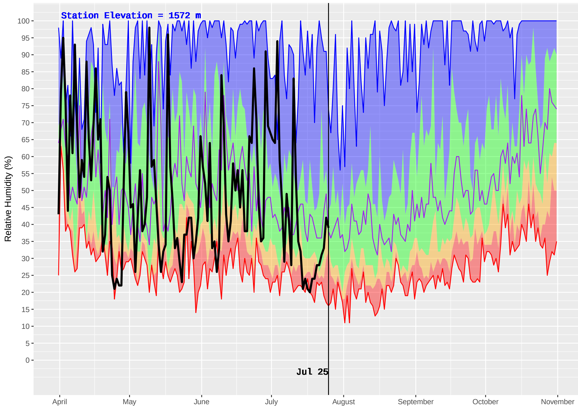
NEGRO CREEK (789) : Historical (2001–2016) and Current (2018) Noon Relative Humidity
